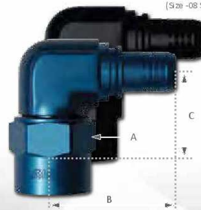
90° Aluminum (Size -08 Shown)
