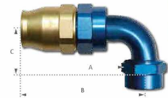
90° Aluminum (Size -16 Shown)
