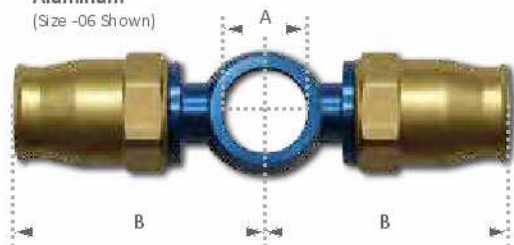
Aluminum (Size -06 Shown)
