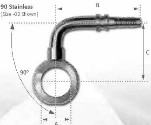
90° Banjo - Side Bend
