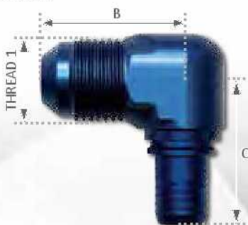
90° Aluminum (Size -08 Shown)
