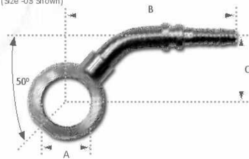
50° Stainless (Size -03 Shown)
