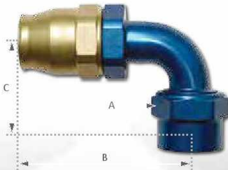
90° Aluminum (Size -10 Shown)
