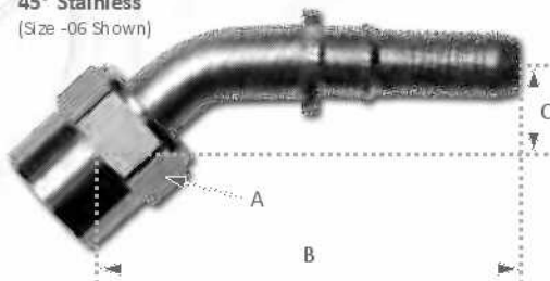
45° Stainless (Size -06 Shown)
