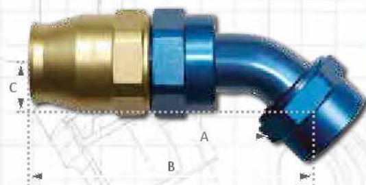
45° Aluminum (Size -16 Shown)
