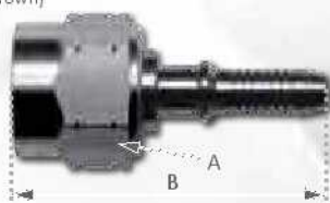
Stainless (Size -04 Shown)
