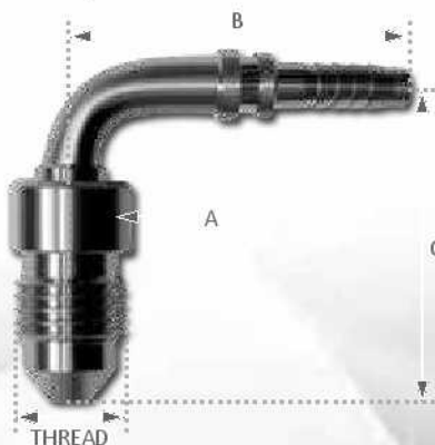
90° Stainless (Size -03 Shown)
