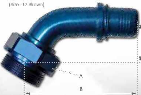
60° Aluminum (Size -12 Shown)
