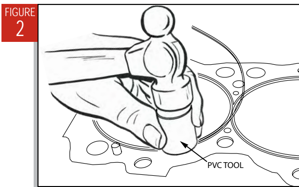
Seat the wire using the PVC tool provided in kit #31542. This will evenly distribute hammer blows and prevent flattening the wire.
