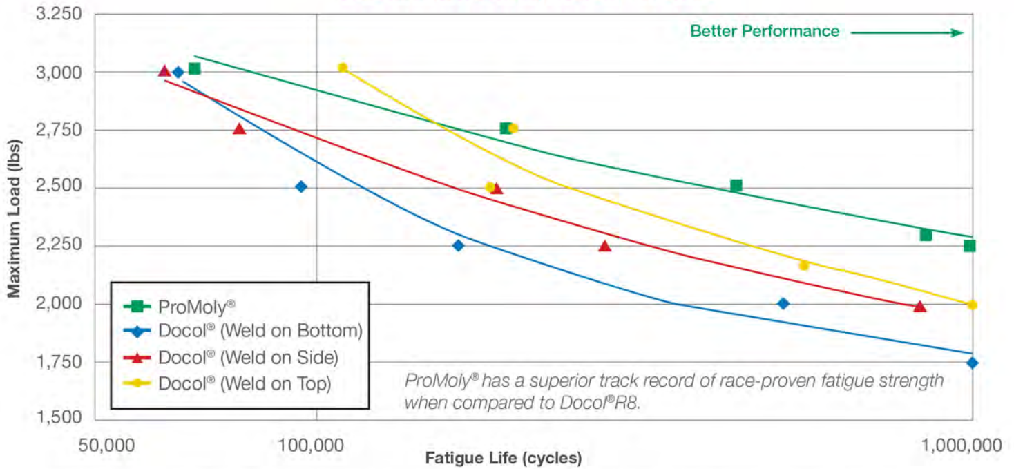
LOAD LIFE DATA CURVES, PROMOLY® vs DOCOL®
