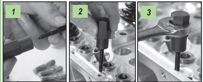
1 - Insert stud into correct size installer.
