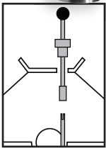
Fig. 1 Insert depth gauge in place of distributor. Bottom out in oil pump drive.
