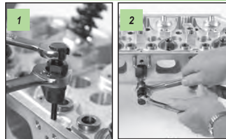
1 - Place the remover over the stud to be removed. Using 2 wrenches, back the stud out of the head.
