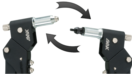
QUICKSWITCH 1 2 3 3 STEPS DISMOUNT AND 3 STEPS ASSEMBLY
