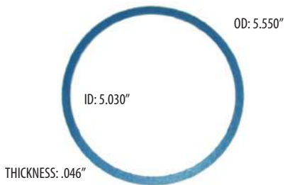
AIR CLEANER GASKET G702 BLACK STANDARD G702BL BLUE NON-STICK G702RD RED NON-STICK
