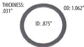
THICKNESS: .031" OD: 1.062" FUEL FITTING WASHER G778 RUBBER COATED ALUMINUM
