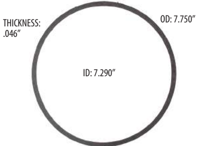
AIR CLEANER GASKET - DOMINATOR G1889 STANDARD MATERIAL - BLACK
