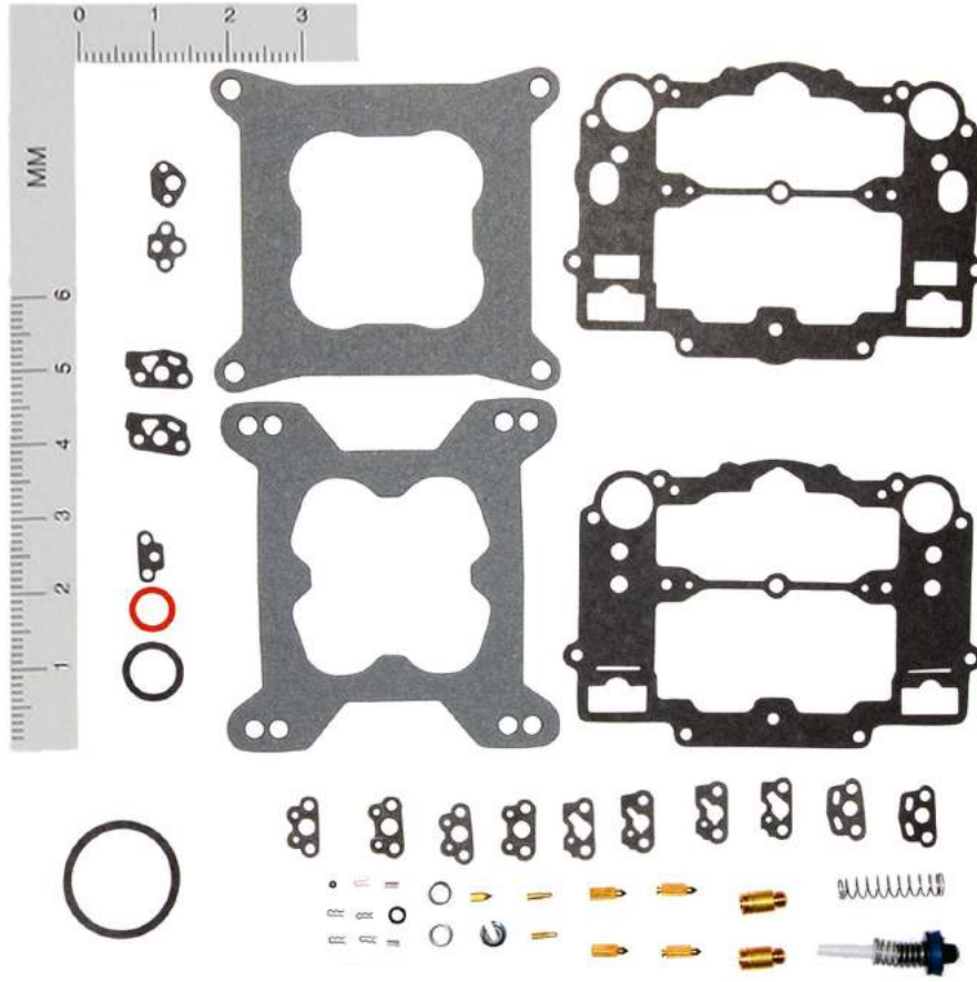
CARTER - SQUARE FLANGE/PERFORMANCE EQUIPPED 15881A
