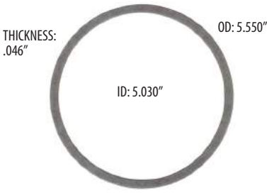
AIR CLEANER GASKET G702 STANDARD MATERIAL - BLACK G702BL NON-STICK - BLUE
