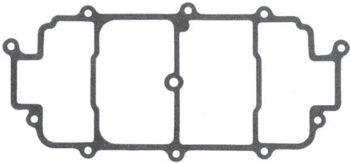
AIR HORN GASKET G1620 STANDARD MATERIAL - BLACK G1620BL NON-STICK - BLUE
