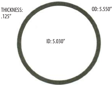
AIR CLEANER GASKET G1857 STANDARD MATERIAL - BLACK
